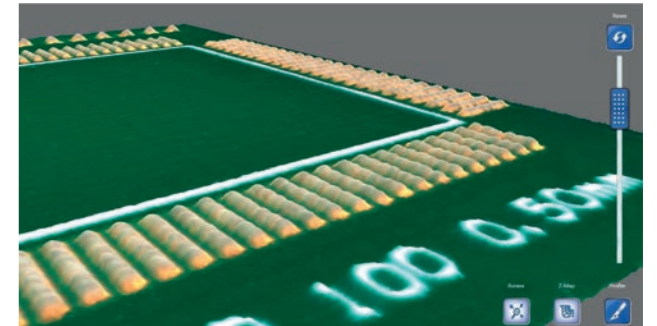
Inspection of jetted paste deposits.
